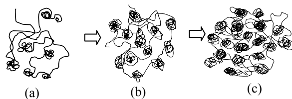
Fig. 3. The Growth of TiO 2 Nuclei in the Sol as a Result of Hydrolysis and Condensation Reactions with R_w of: (a) 0.85; (b) 2.00 and (c) 3.50
